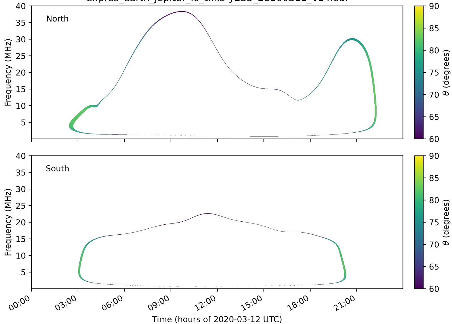
expres_earth_jupiter_io_txka-y235_20200312_v14.cdf
