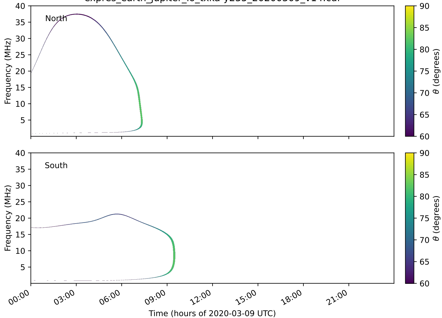
expres_earth_jupiter_io_txka-y235_20200309_v14.cdf
