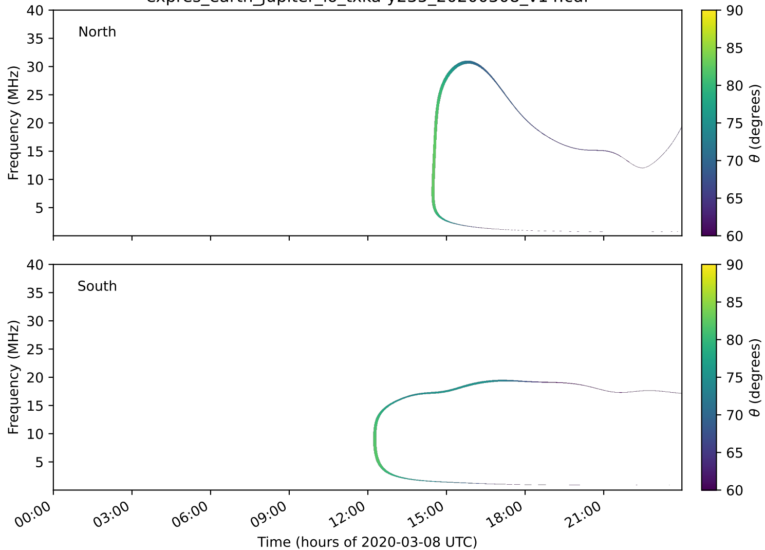
expres_earth_jupiter_io_txka-y235_20200308_v14.cdf
