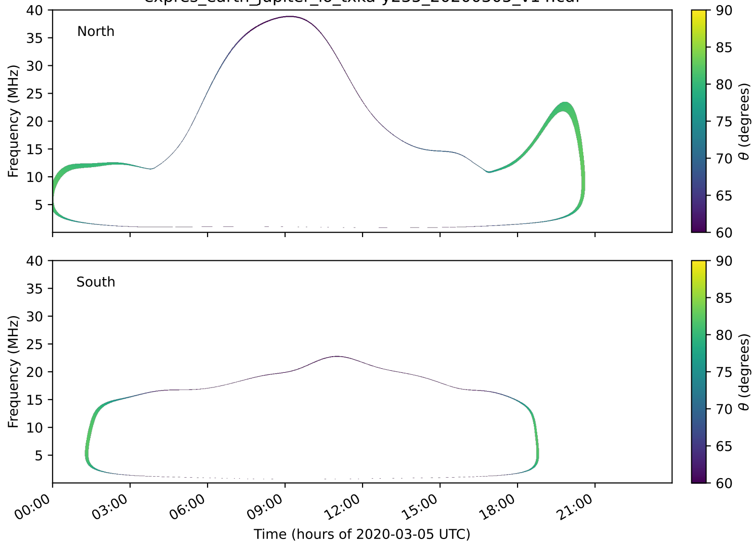
expres_earth_jupiter_io_txka-y235_20200305_v14.cdf
