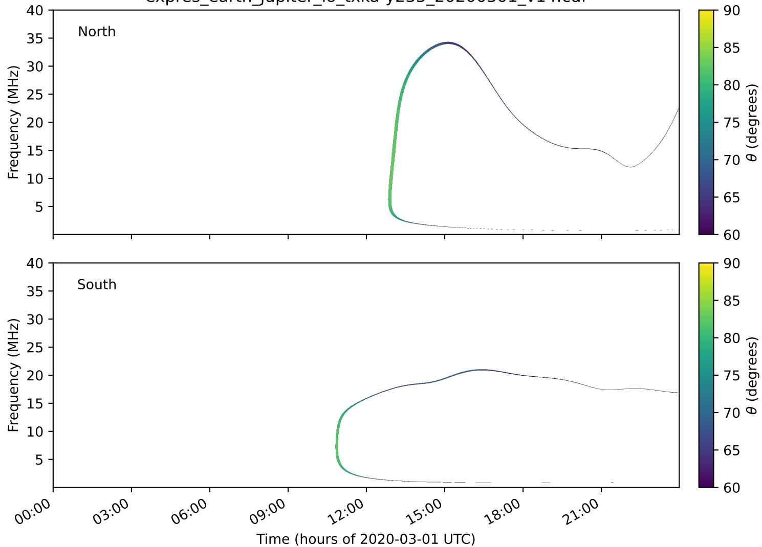
expres_earth_jupiter_io_txka-y235_20200301_v14.cdf
