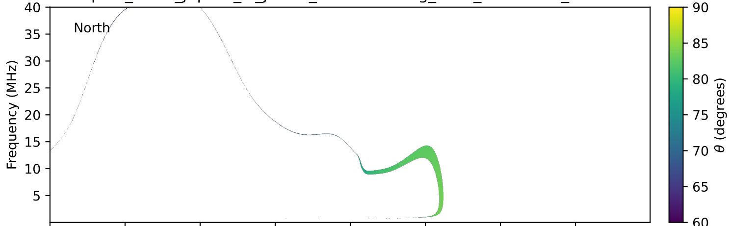
expres_earth_jupiter_io_jrm33_lossc-wid1deg_3kev_20200330_v11.cdf
