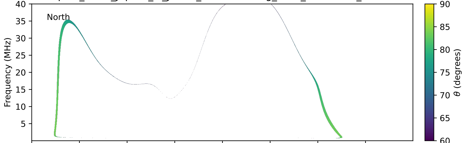
expres_earth_jupiter_io_jrm33_lossc-wid1deg_3kev_20200328_v11.cdf
