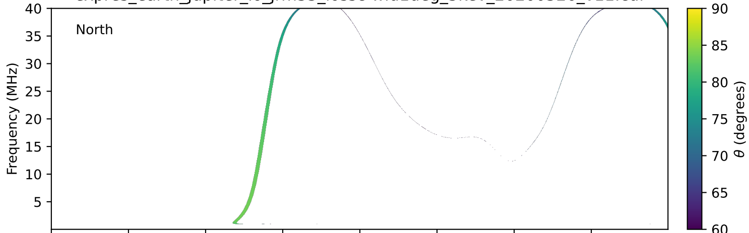
expres_earth_jupiter_io_jrm33_lossc-wid1deg_3kev_20200326_v11.cdf
