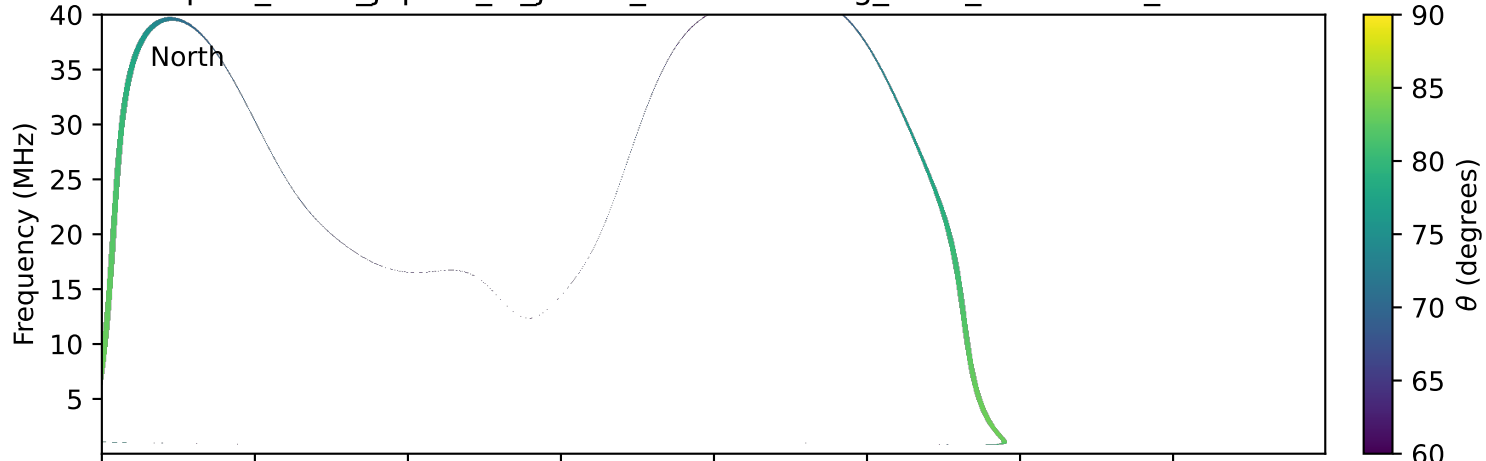
expres_earth_jupiter_io_jrm33_lossc-wid1deg_3kev_20200321_v11.cdf
