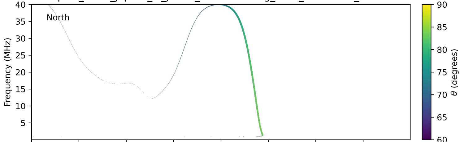
expres_earth_jupiter_io_jrm33_lossc-wid1deg_3kev_20200307_v11.cdf
