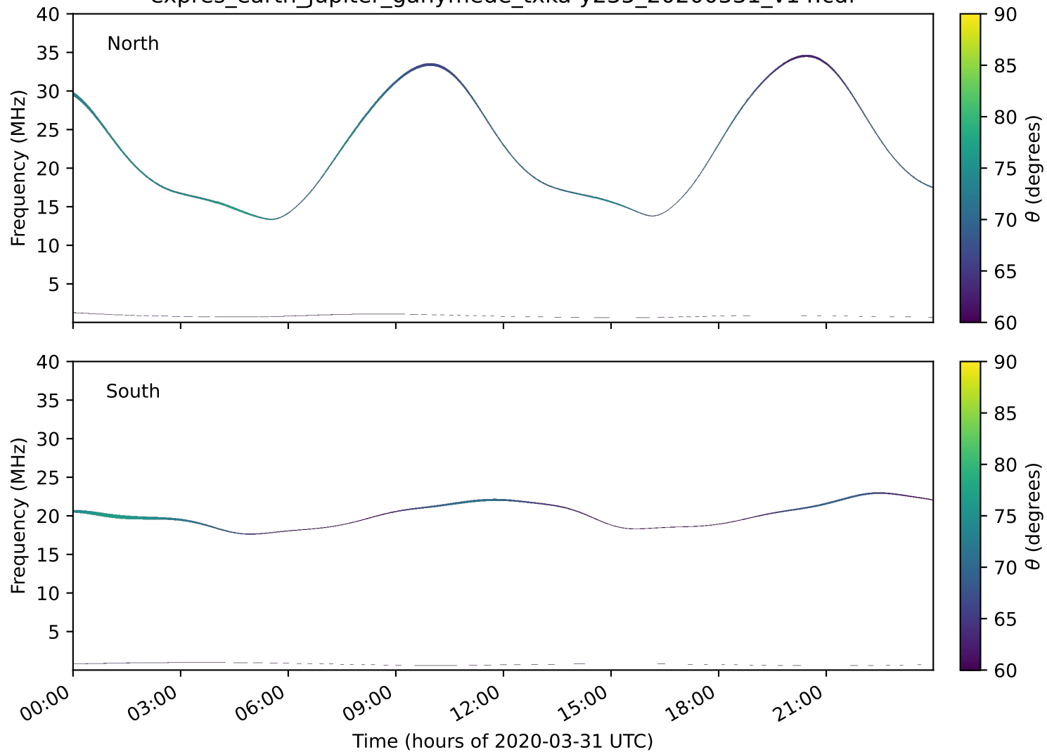
expres_earth_jupiter_ganymede_txka-y235_20200331_v14.cdf
