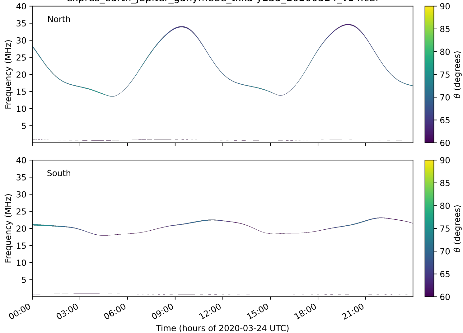
expres_earth_jupiter_ganymede_txka-y235_20200324_v14.cdf
