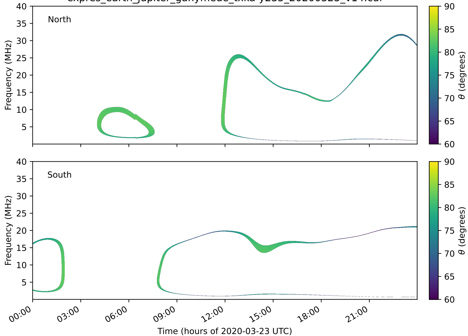
expres_earth_jupiter_ganymede_txka-y235_20200323_v14.cdf
