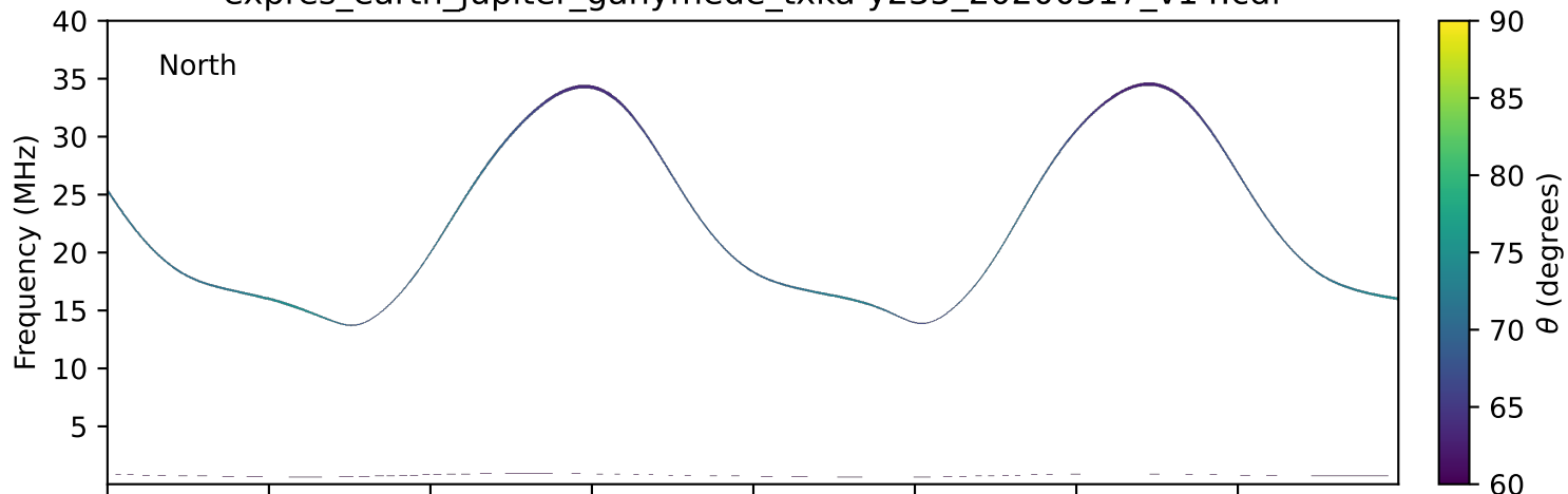
expres_earth_jupiter_ganymede_txka-y235_20200317_v14.cdf
