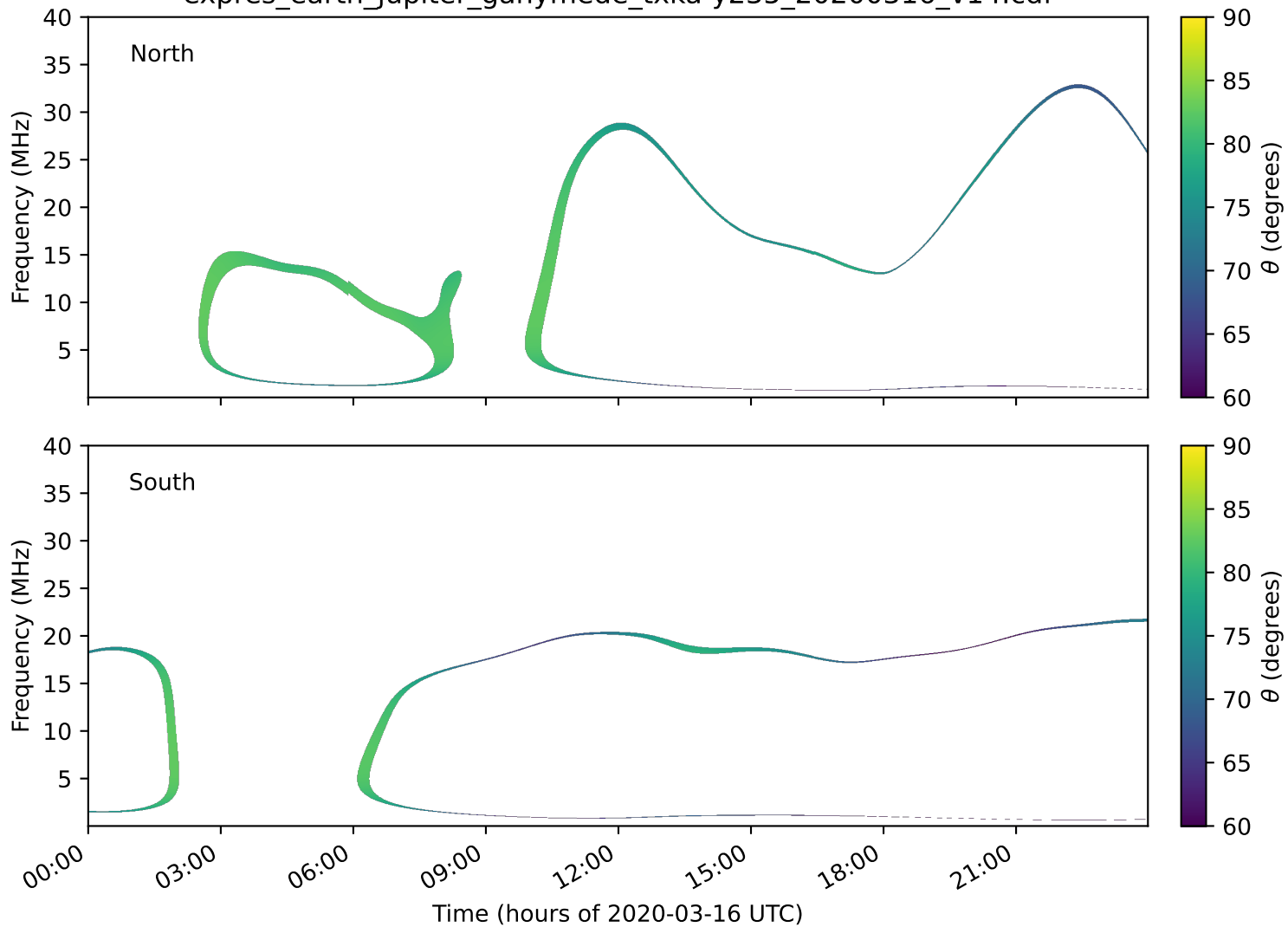
expres_earth_jupiter_ganymede_txka-y235_20200316_v14.cdf
