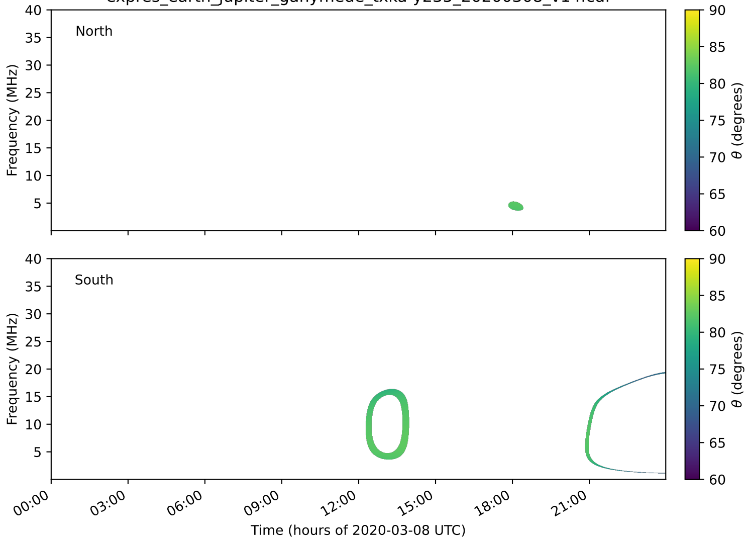
expres_earth_jupiter_ganymede_txka-y235_20200308_v14.cdf
