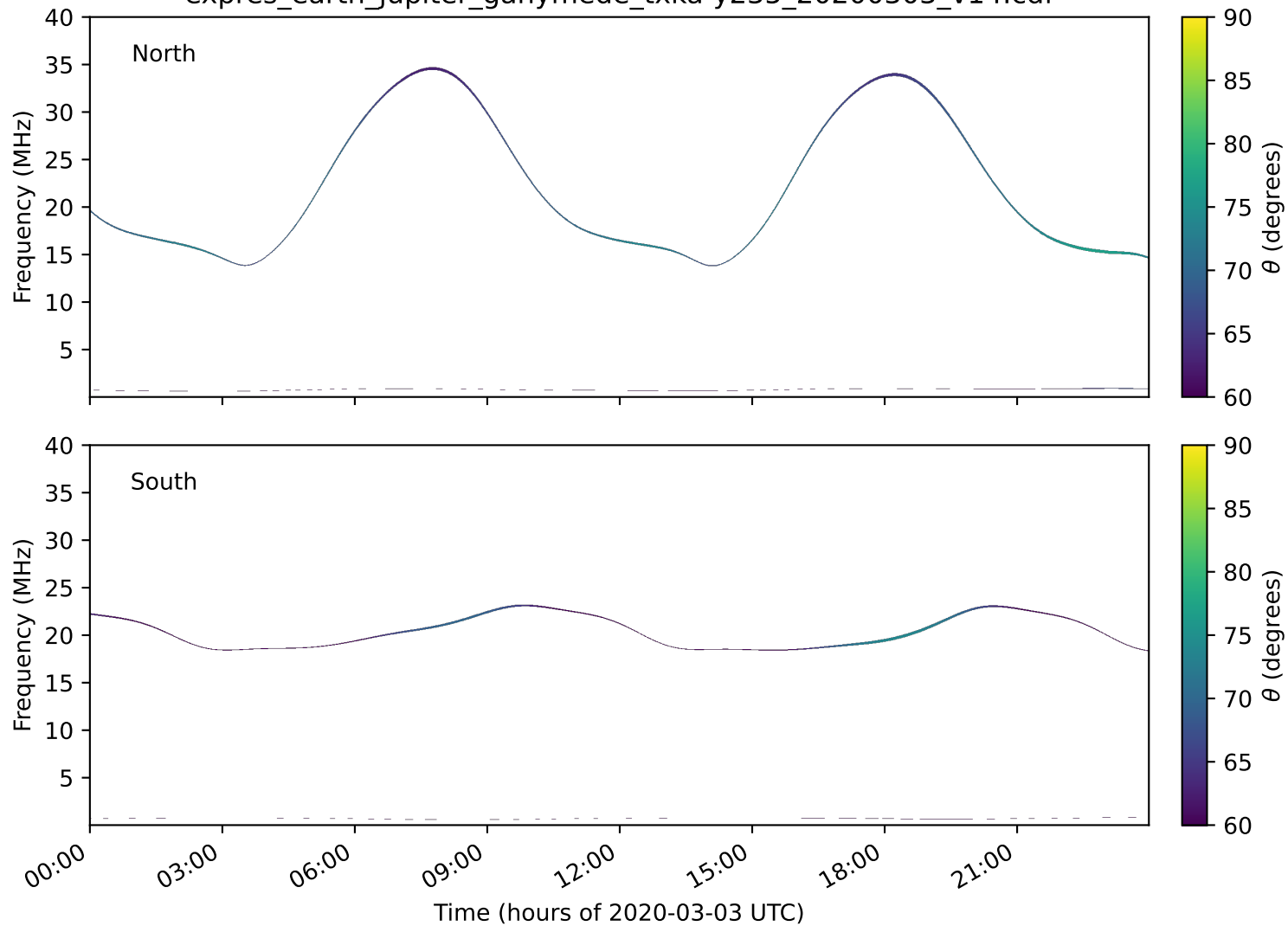
expres_earth_jupiter_ganymede_txka-y235_20200303_v14.cdf
