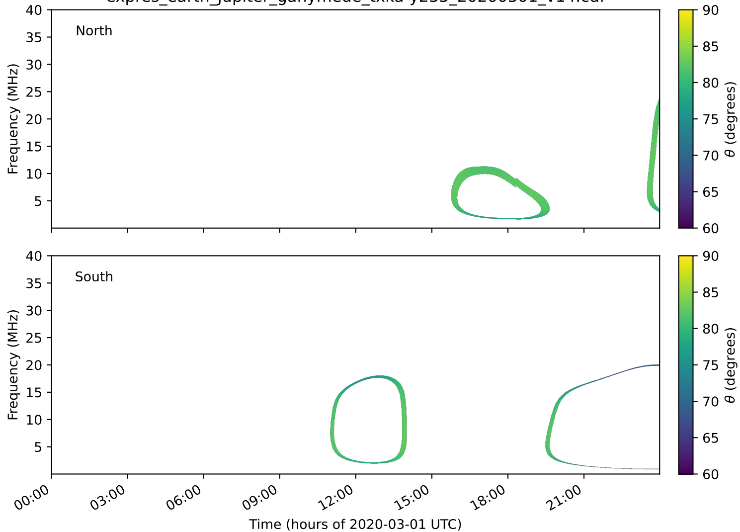
expres_earth_jupiter_ganymede_txka-y235_20200301_v14.cdf
