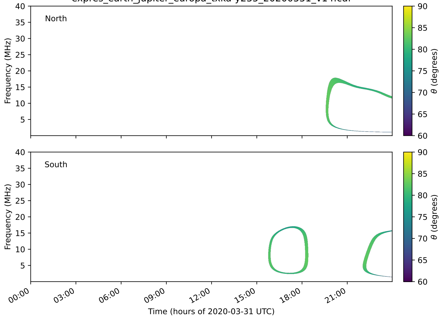
expres_earth_jupiter_europa_txka-y235_20200331_v14.cdf
