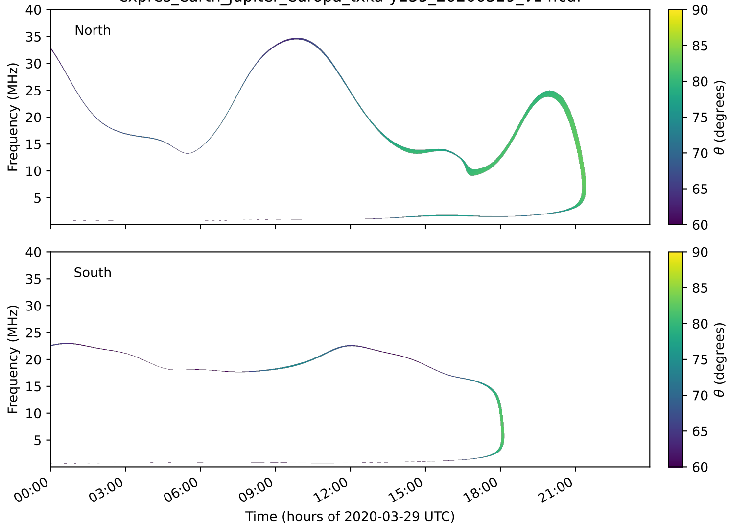
expres_earth_jupiter_europa_txka-y235_20200329_v14.cdf
