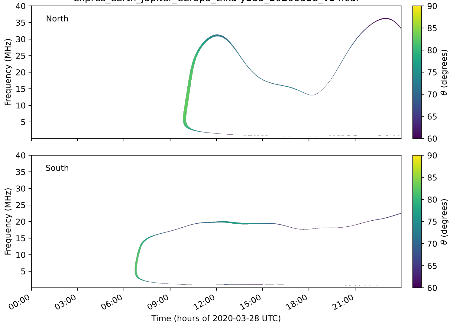
expres_earth_jupiter_europa_txka-y235_20200328_v14.cdf
