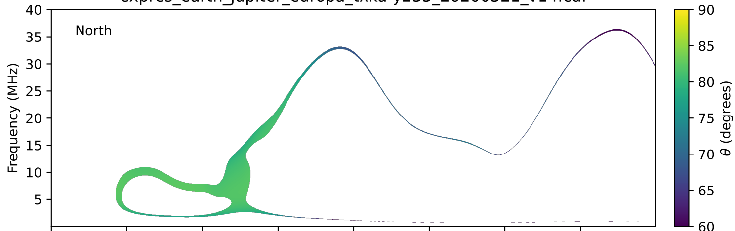
expres_earth_jupiter_europa_txka-y235_20200321_v14.cdf
