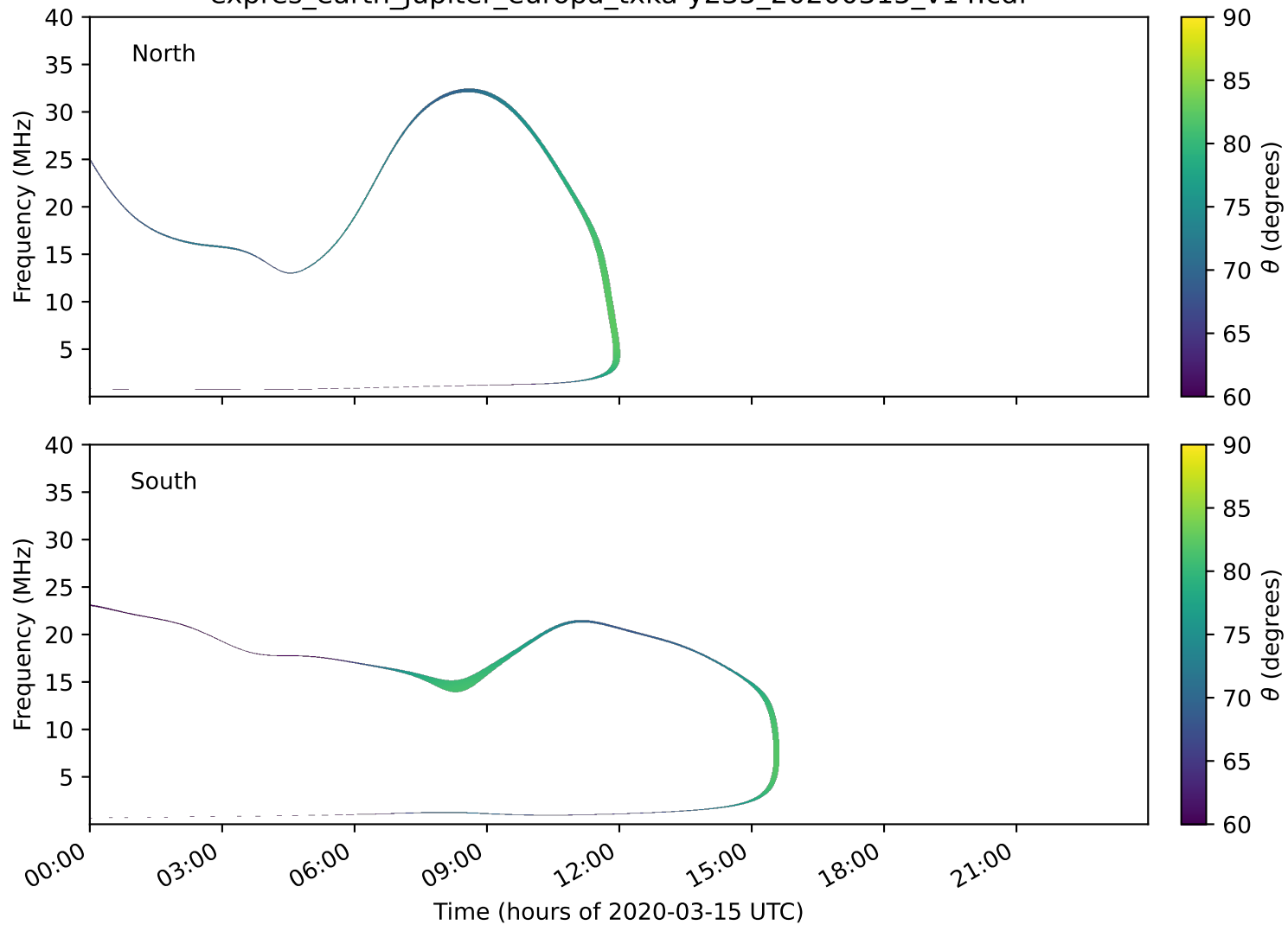
expres_earth_jupiter_europa_txka-y235_20200315_v14.cdf
