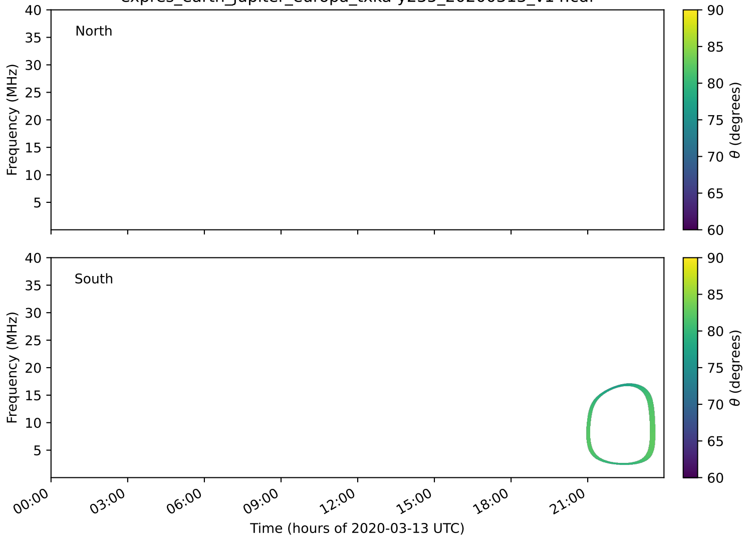
expres_earth_jupiter_europa_txka-y235_20200313_v14.cdf
