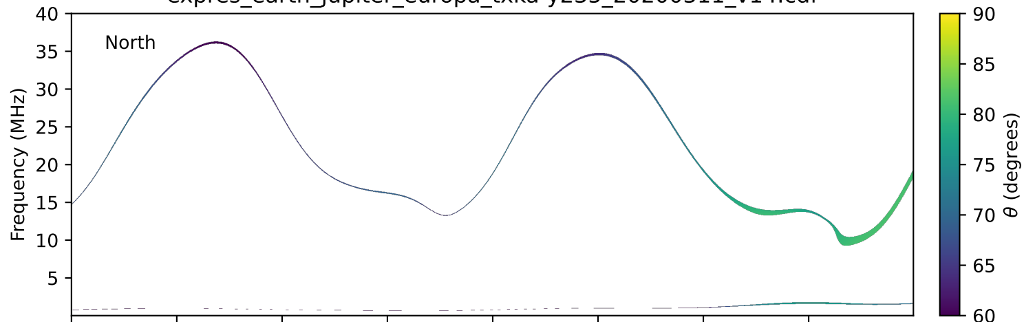
expres_earth_jupiter_europa_txka-y235_20200311_v14.cdf
