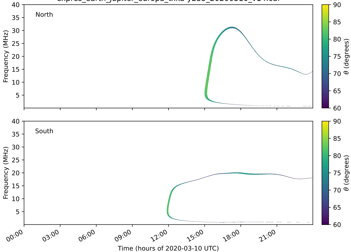
expres_earth_jupiter_europa_txka-y235_20200310_v14.cdf
