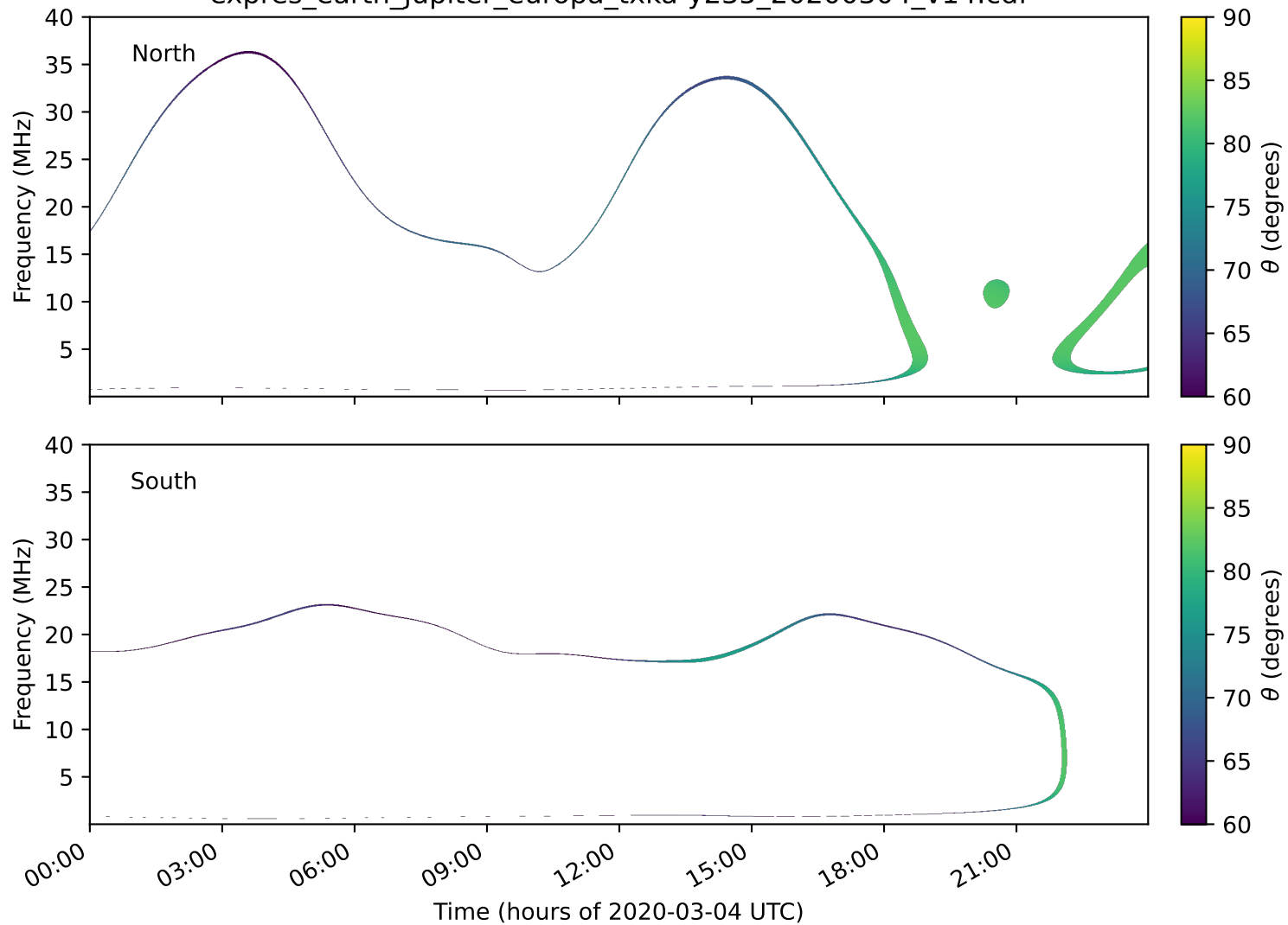
expres_earth_jupiter_europa_txka-y235_20200304_v14.cdf
