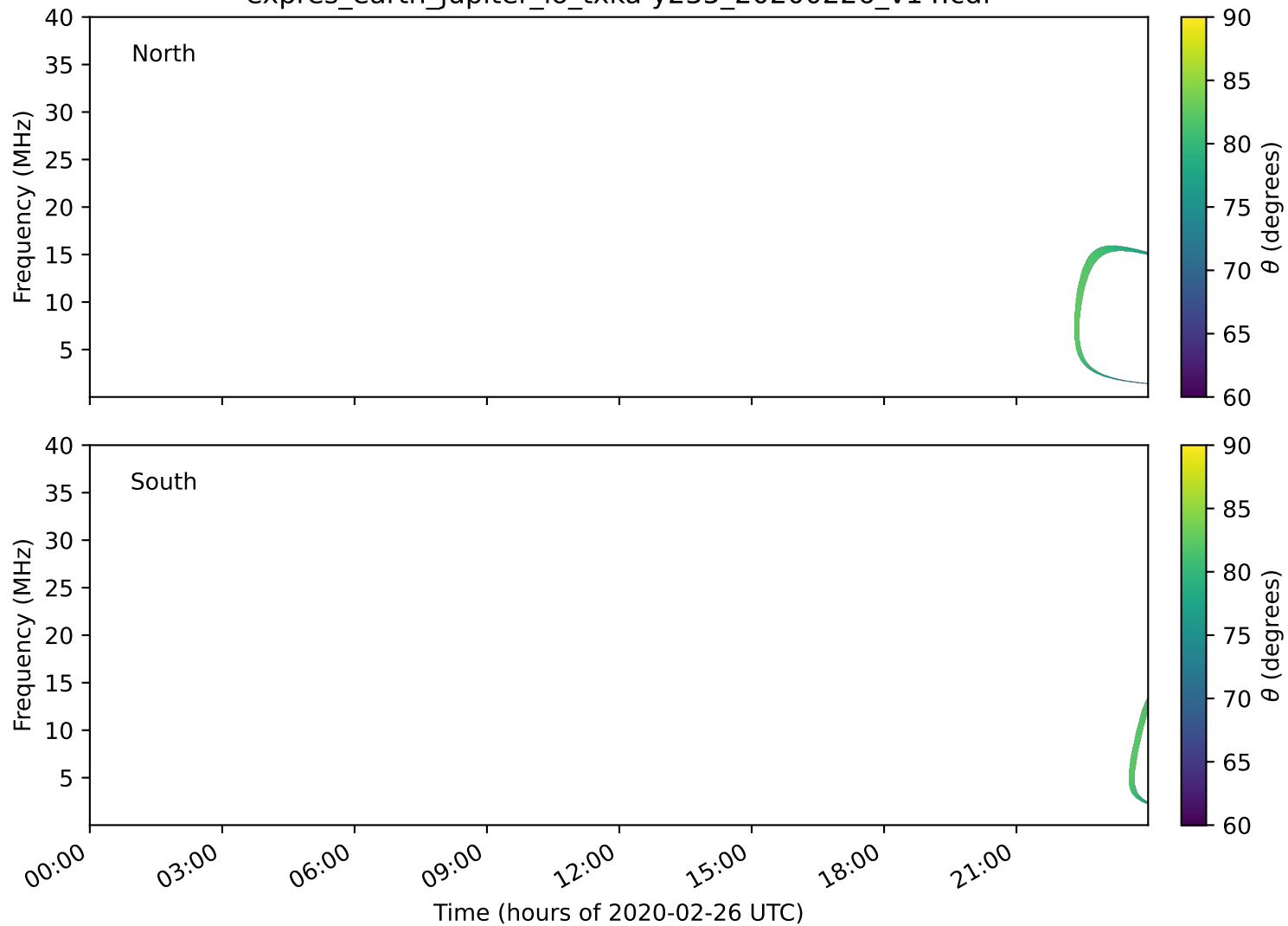
expres_earth_jupiter_io_txka-y235_20200226_v14.cdf
