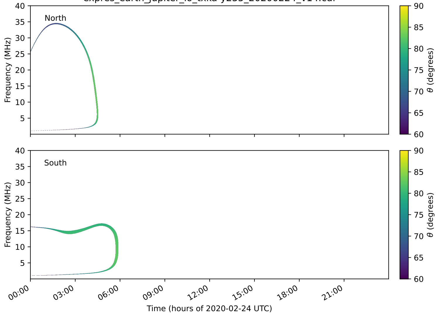
expres_earth_jupiter_io_txka-y235_20200224_v14.cdf
