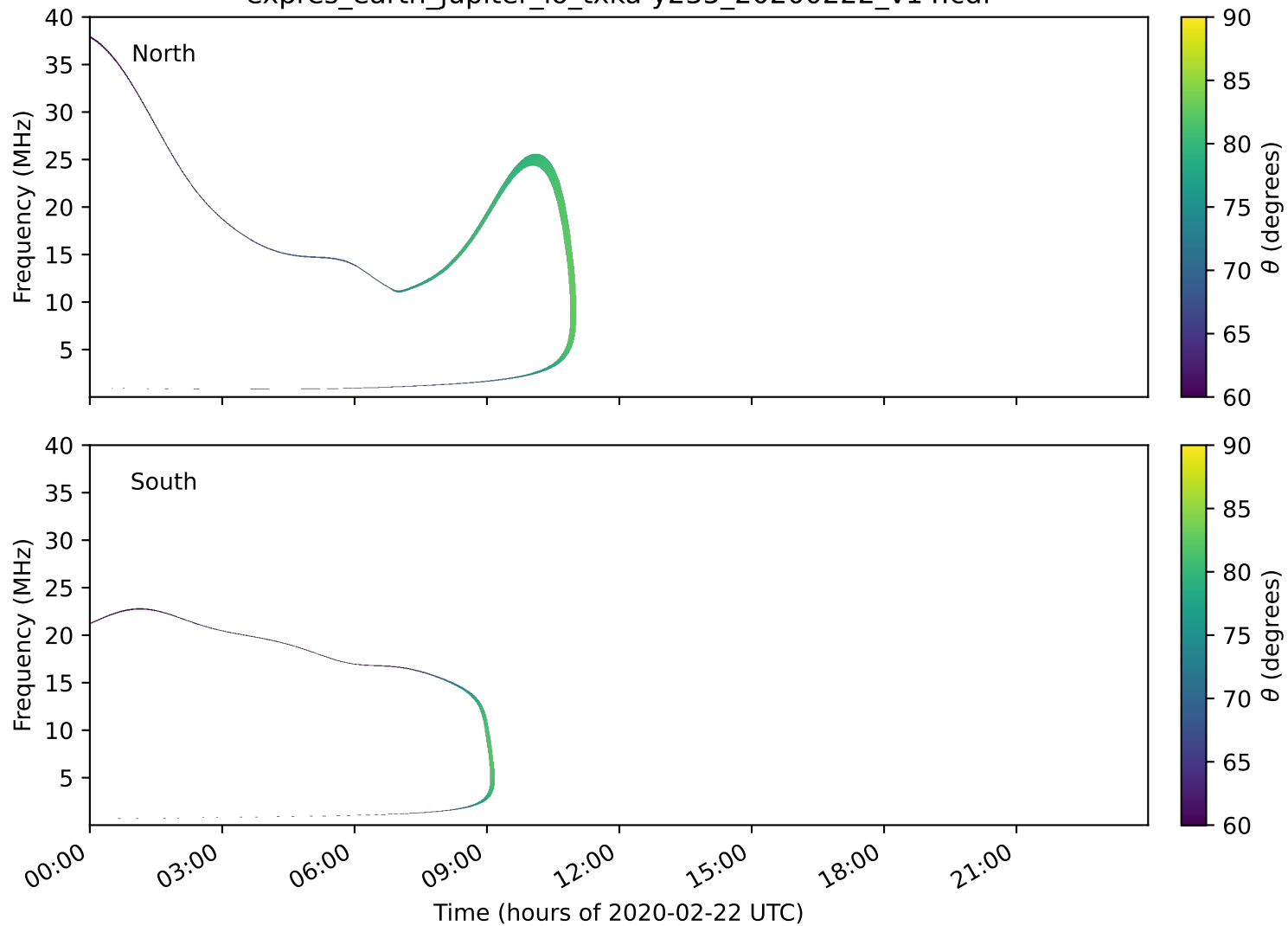
expres_earth_jupiter_io_txka-y235_20200222_v14.cdf
