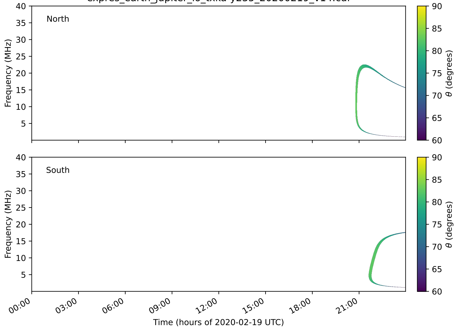
expres_earth_jupiter_io_txka-y235_20200219_v14.cdf
