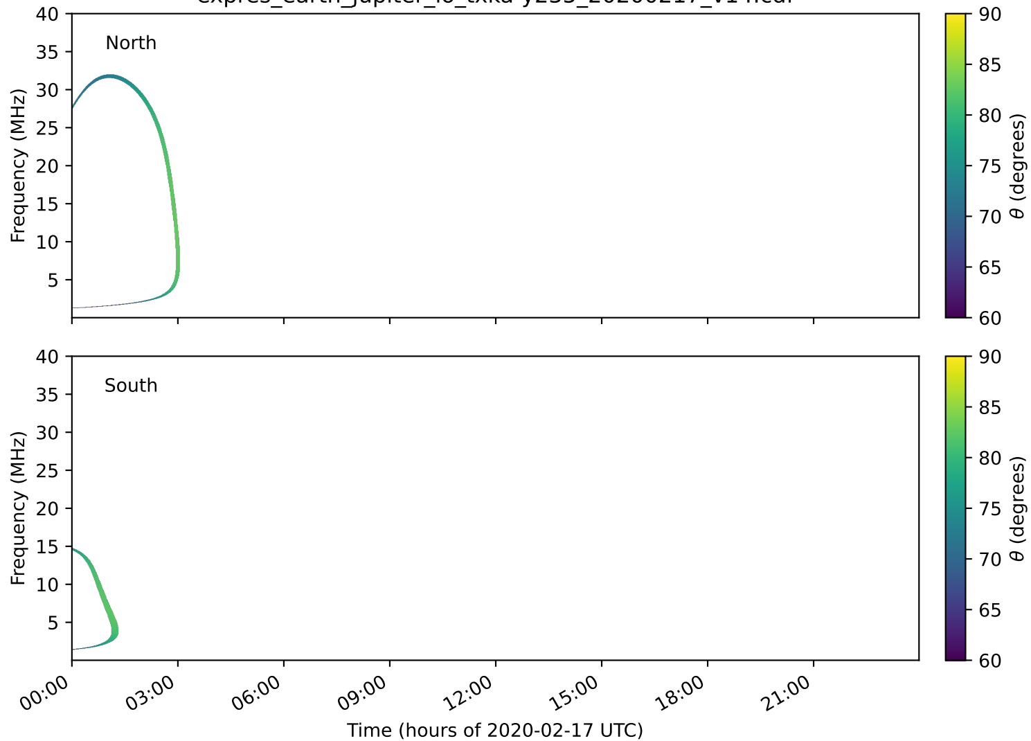
expres_earth_jupiter_io_txka-y235_20200217_v14.cdf
