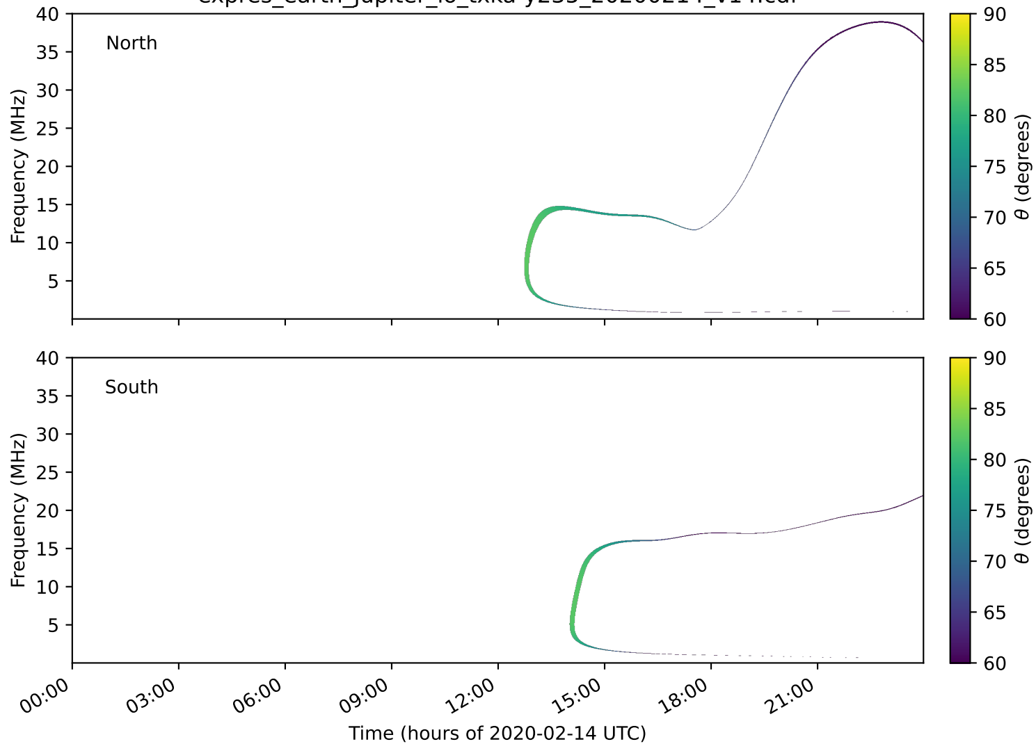
expres_earth_jupiter_io_txka-y235_20200214_v14.cdf
