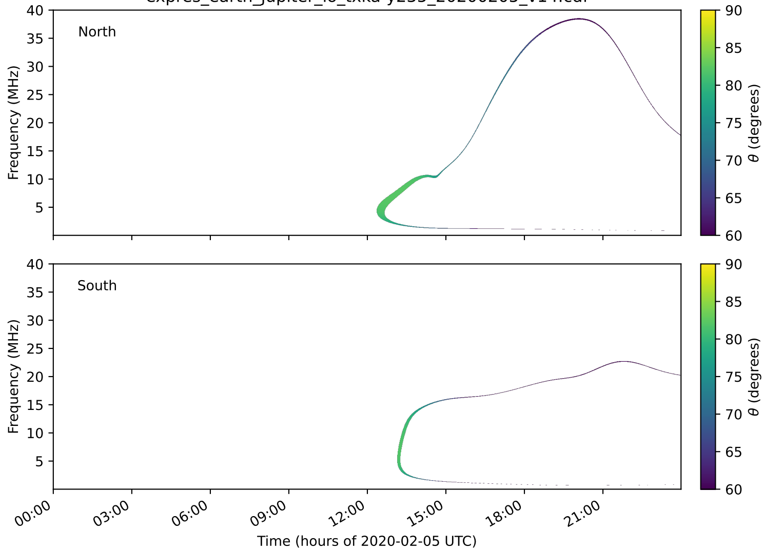
expres_earth_jupiter_io_txka-y235_20200205_v14.cdf
