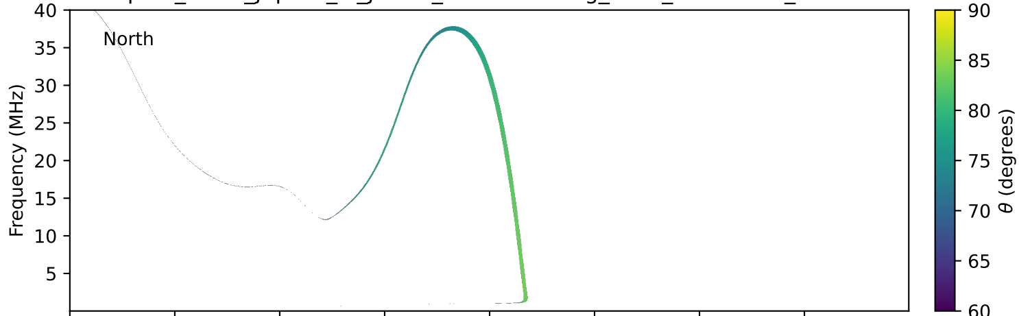
expres_earth_jupiter_io_jrm33_lossc-wid1deg_3kev_20200229_v11.cdf
