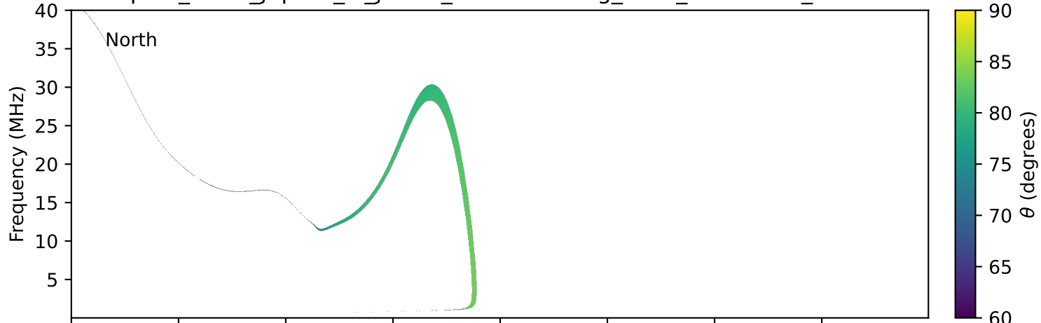
expres_earth_jupiter_io_jrm33_lossc-wid1deg_3kev_20200222_v11.cdf
