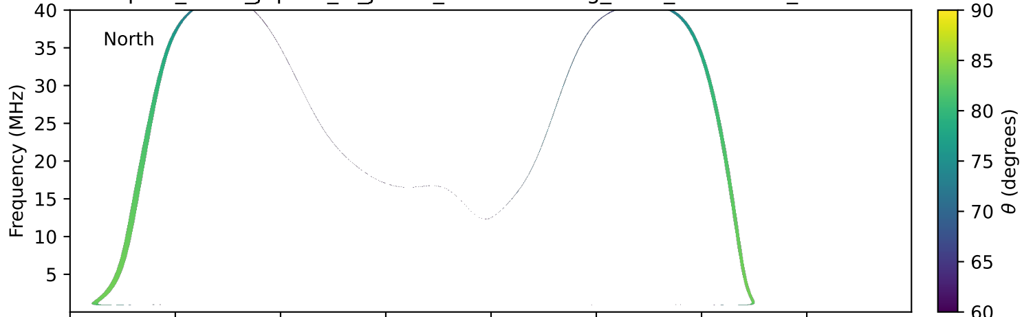
expres_earth_jupiter_io_jrm33_lossc-wid1deg_3kev_20200211_v11.cdf
