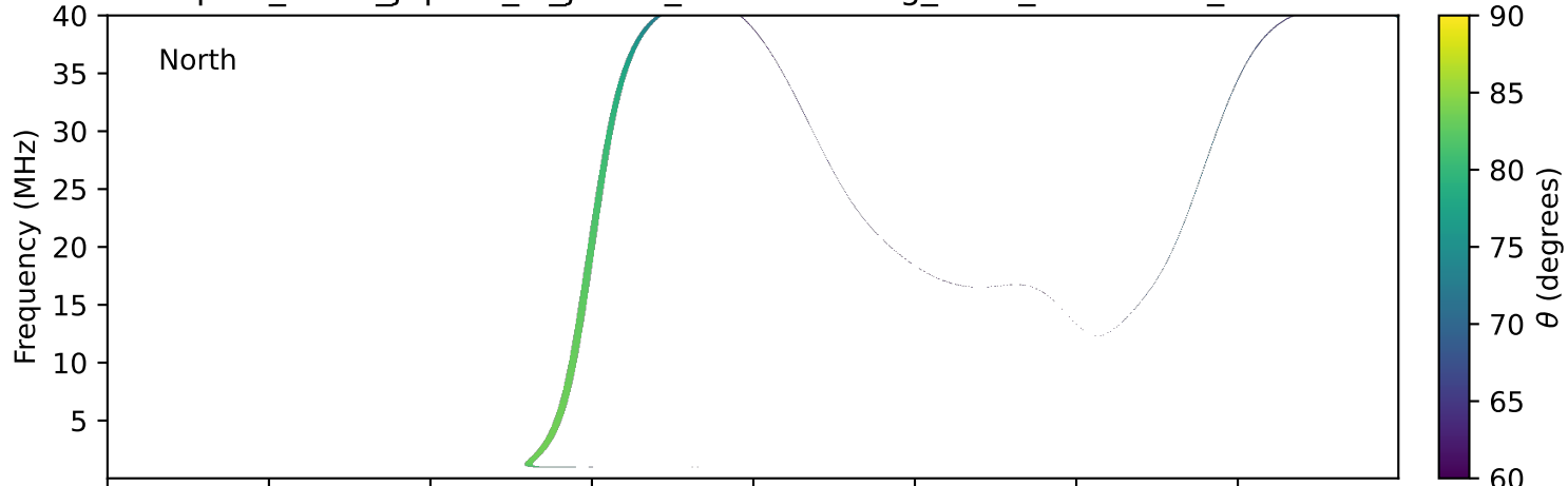
expres_earth_jupiter_io_jrm33_lossc-wid1deg_3kev_20200207_v11.cdf
