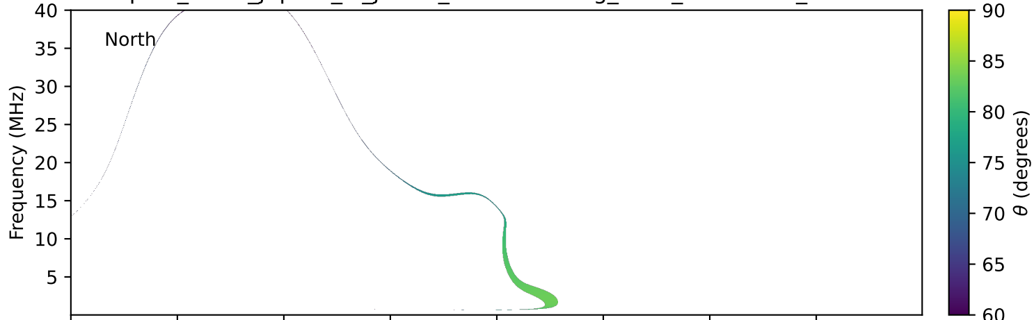
expres_earth_jupiter_io_jrm33_lossc-wid1deg_3kev_20200204_v11.cdf
