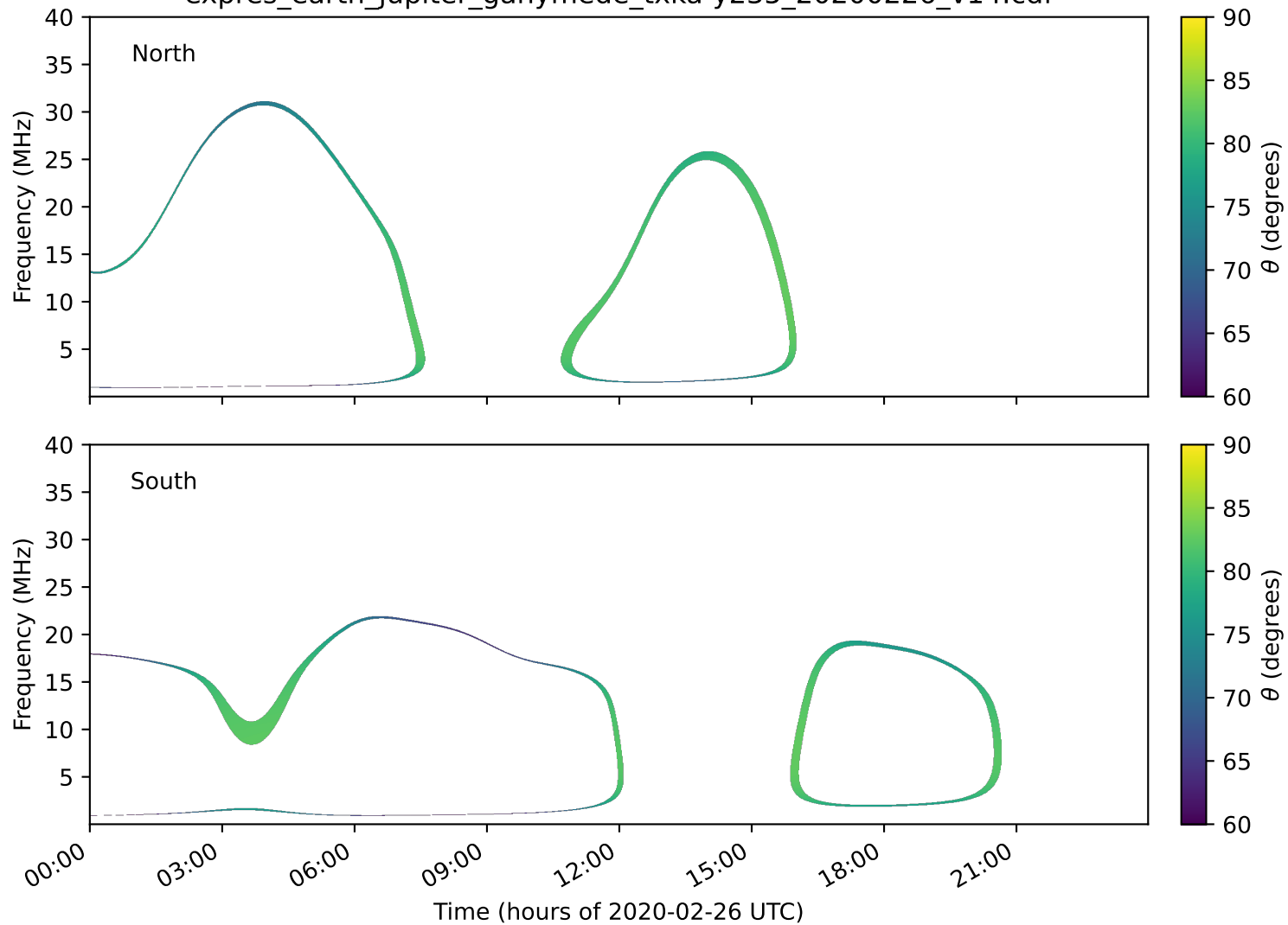
expres_earth_jupiter_ganymede_txka-y235_20200226_v14.cdf
