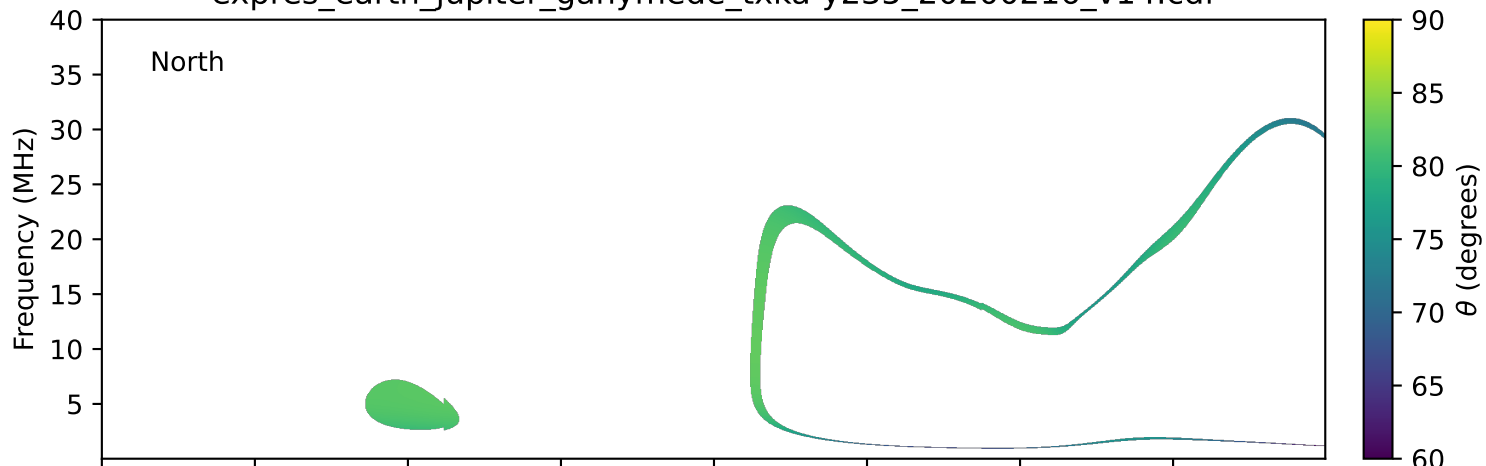
expres_earth_jupiter_ganymede_txka-y235_20200216_v14.cdf
