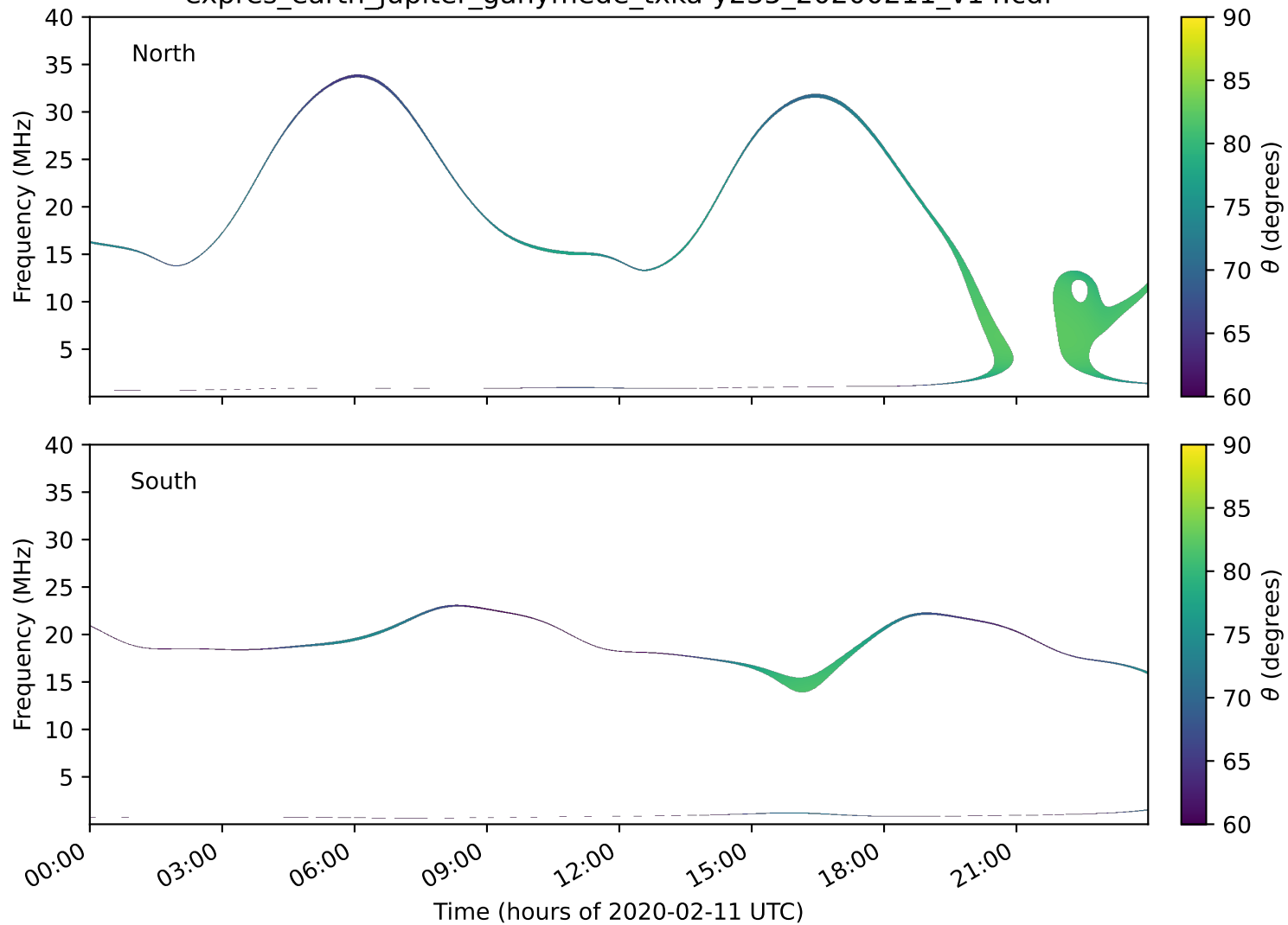
expres_earth_jupiter_ganymede_txka-y235_20200211_v14.cdf
