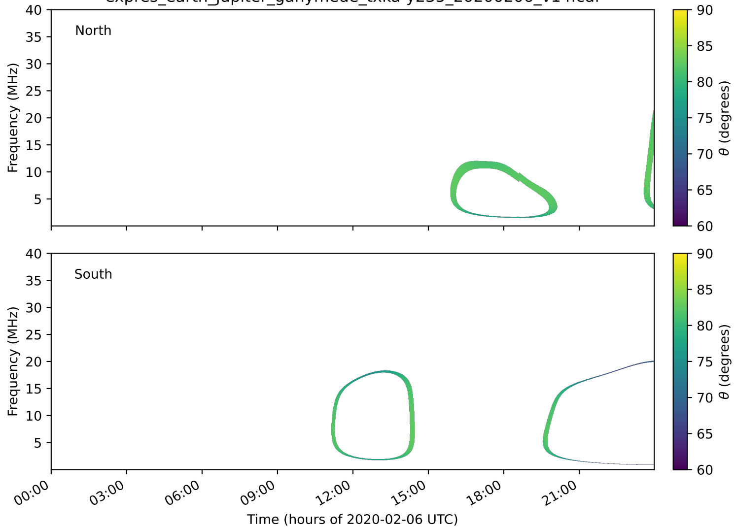
expres_earth_jupiter_ganymede_txka-y235_20200206_v14.cdf
