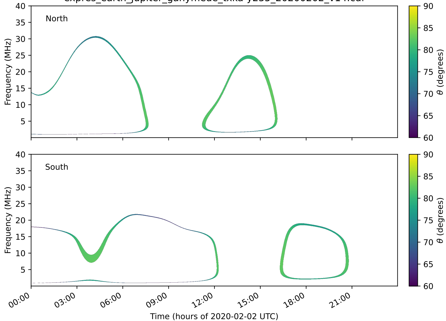
expres_earth_jupiter_ganymede_txka-y235_20200202_v14.cdf
