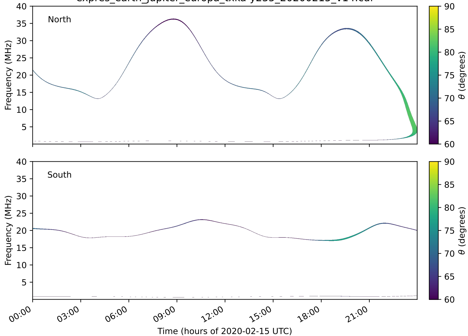
expres_earth_jupiter_europa_txka-y235_20200215_v14.cdf
