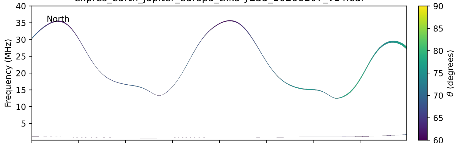
expres_earth_jupiter_europa_txka-y235_20200207_v14.cdf
