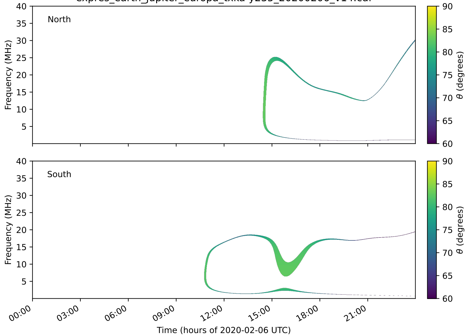
expres_earth_jupiter_europa_txka-y235_20200206_v14.cdf
