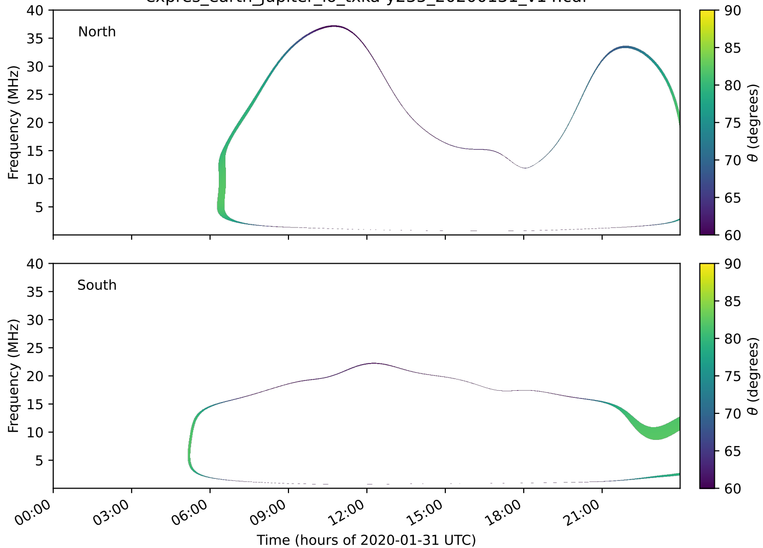
expres_earth_jupiter_io_txka-y235_20200131_v14.cdf
