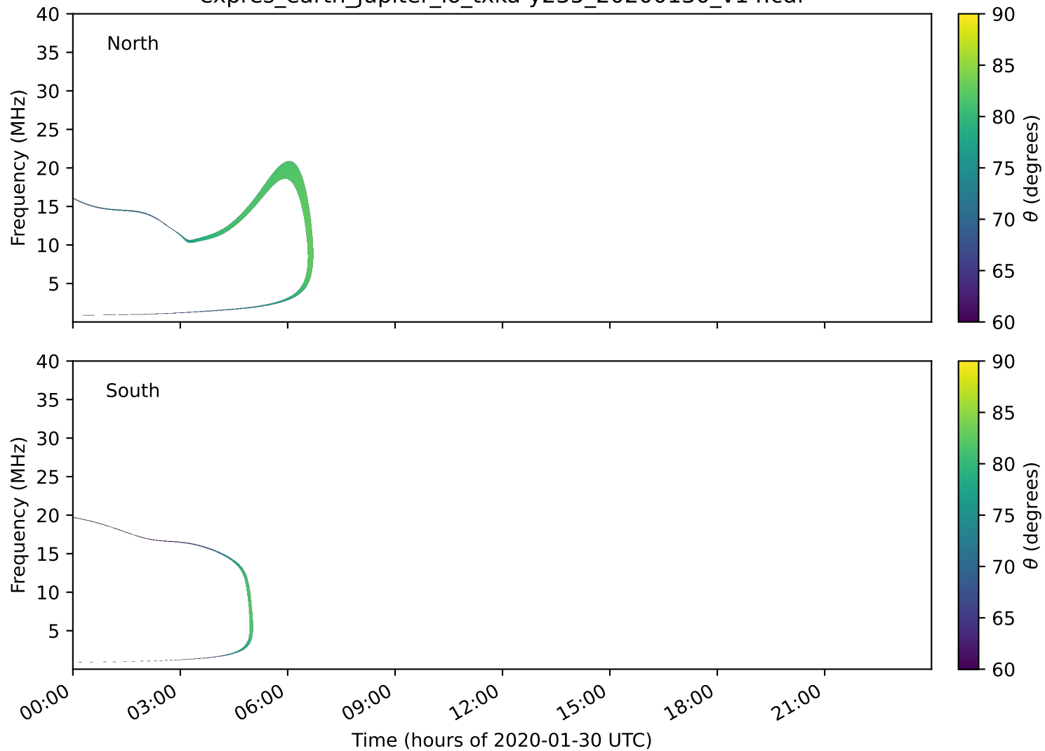
expres_earth_jupiter_io_txka-y235_20200130_v14.cdf
