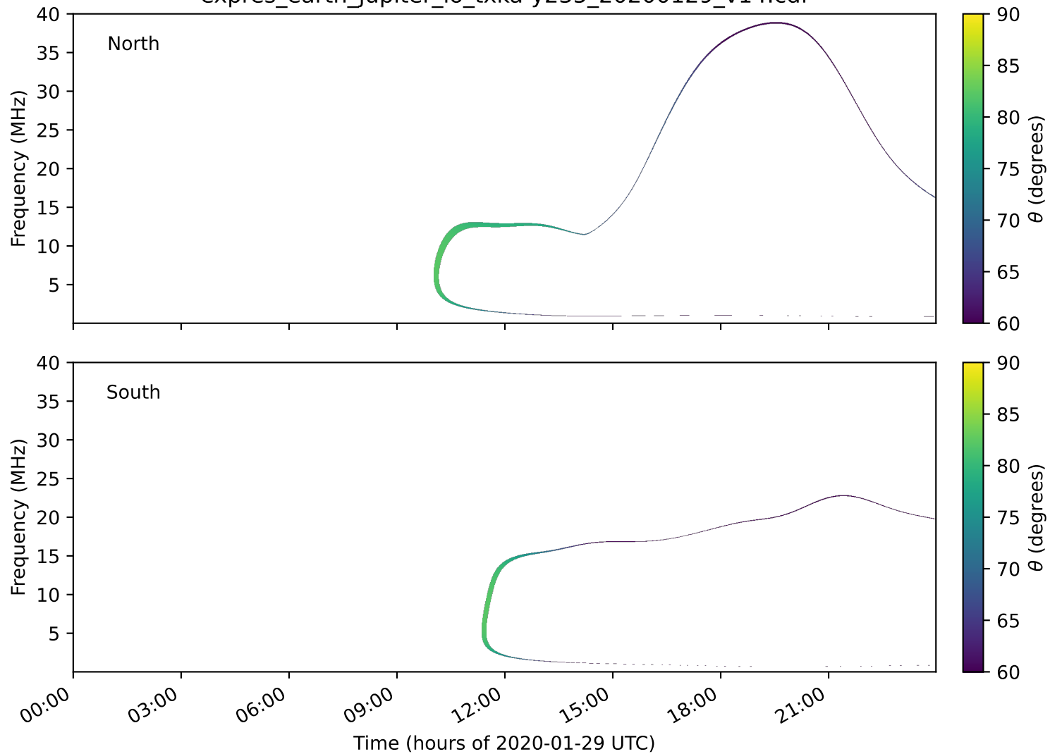
expres_earth_jupiter_io_txka-y235_20200129_v14.cdf
